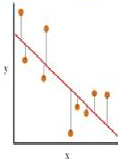
Simple Linear Regression
