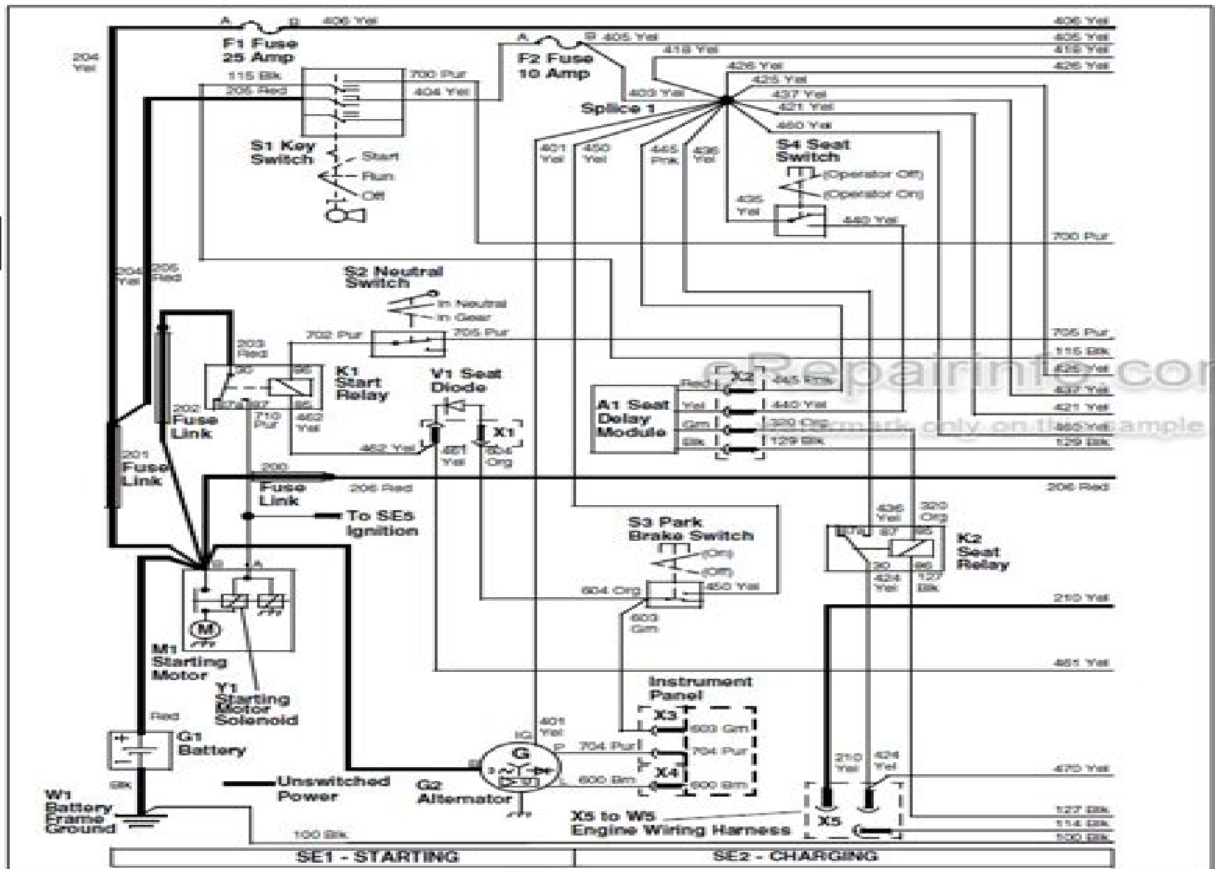
W1 Main Wiring Schematic - Gasoline Engine (Old)
