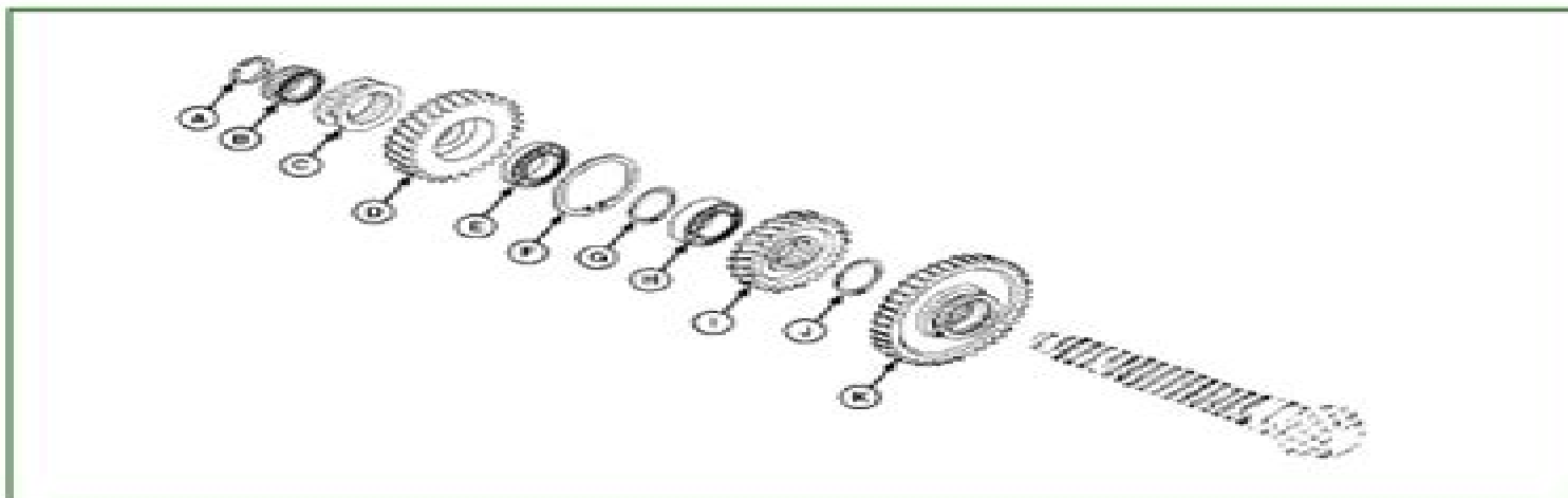
LV11074-UN: MFWD and Range Gears
