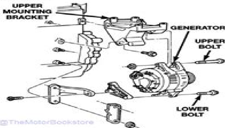
Fig. 4 Remove/Install Generator—2.5L Engine
