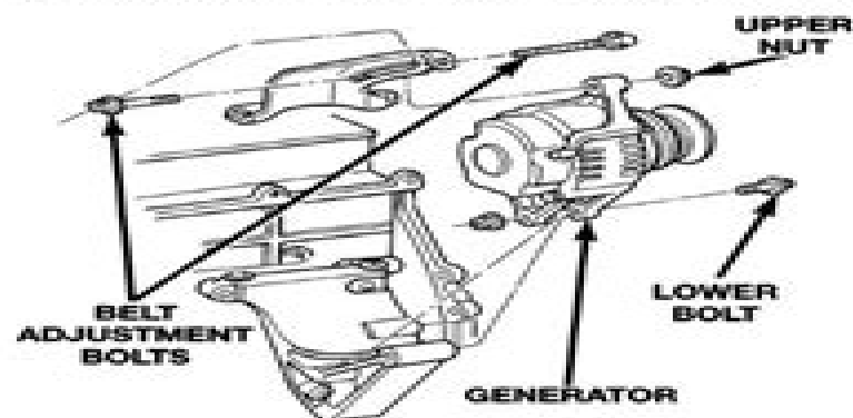
Fig. 6 Remove/Install Generator—4.0L Engine—RHD
