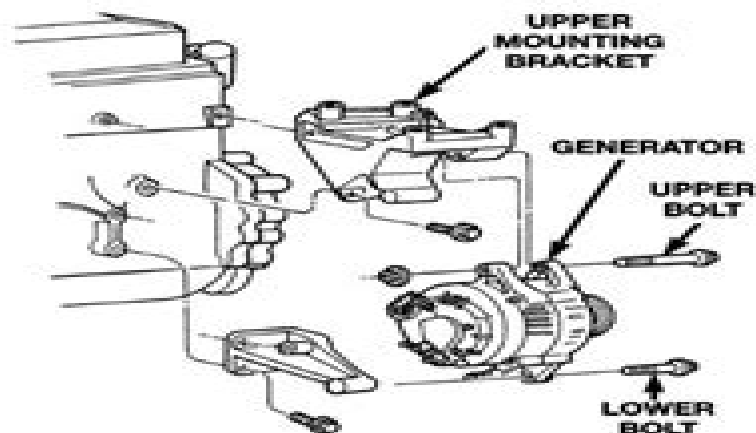
Fig. 5 Remove/Install Generator—4.0L Engine—LHD
