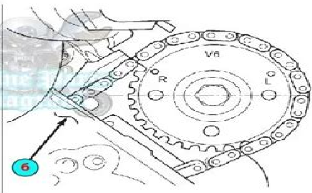
Camshaft Sprocket V6 Marks
