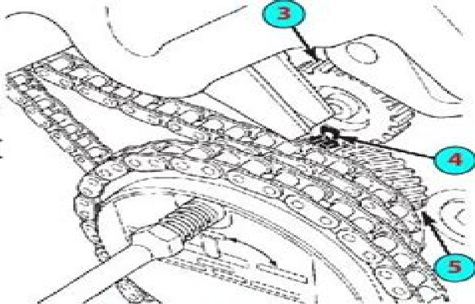
Counterbalance Shaft Alignment Marks
