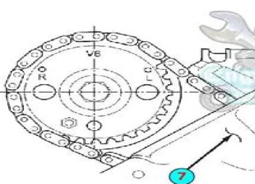
Camshaft Sprocket V6 Marks
