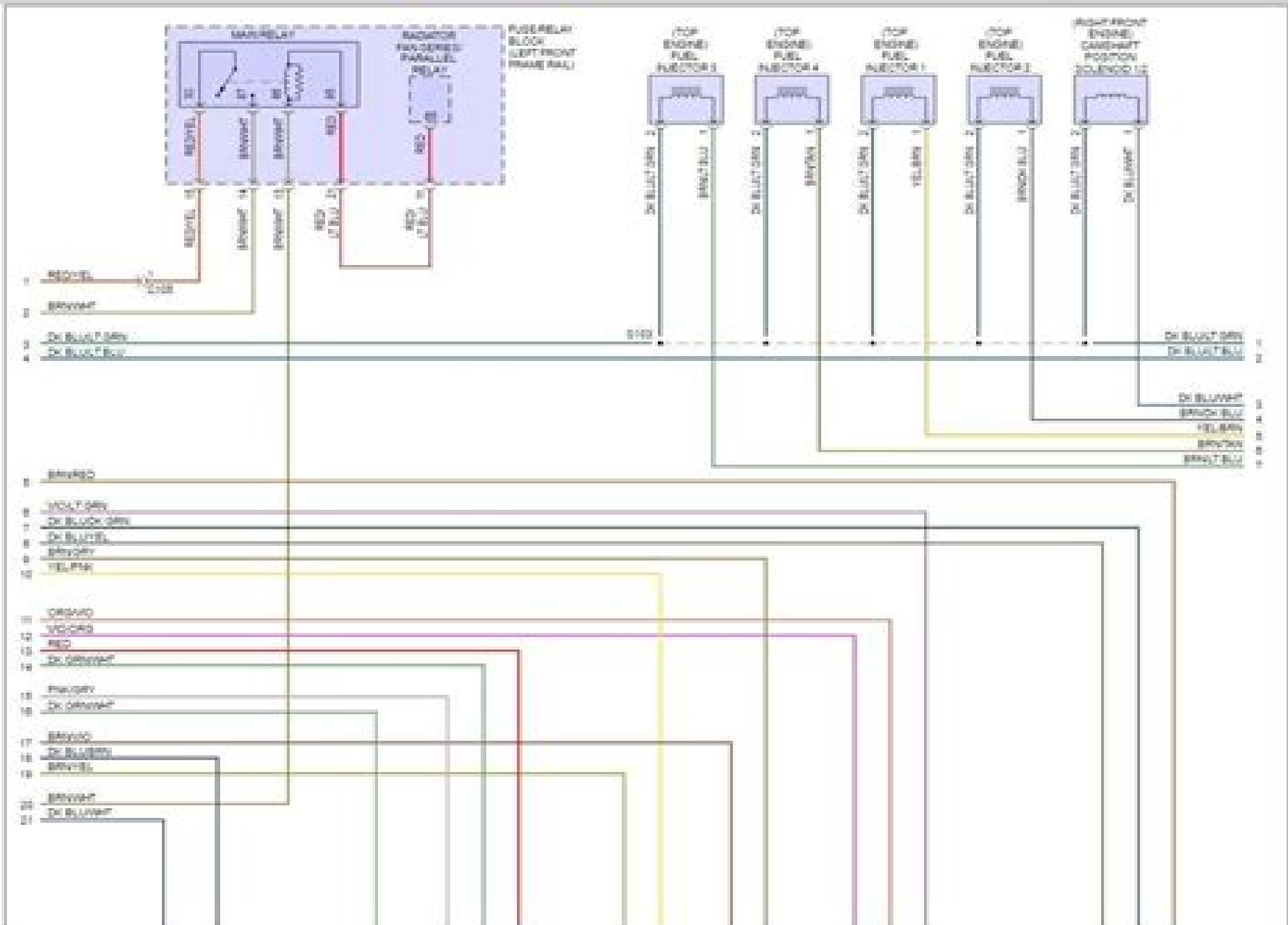
Fig 2: 2.0L, Engine Performance Circuit (2 of 5)
