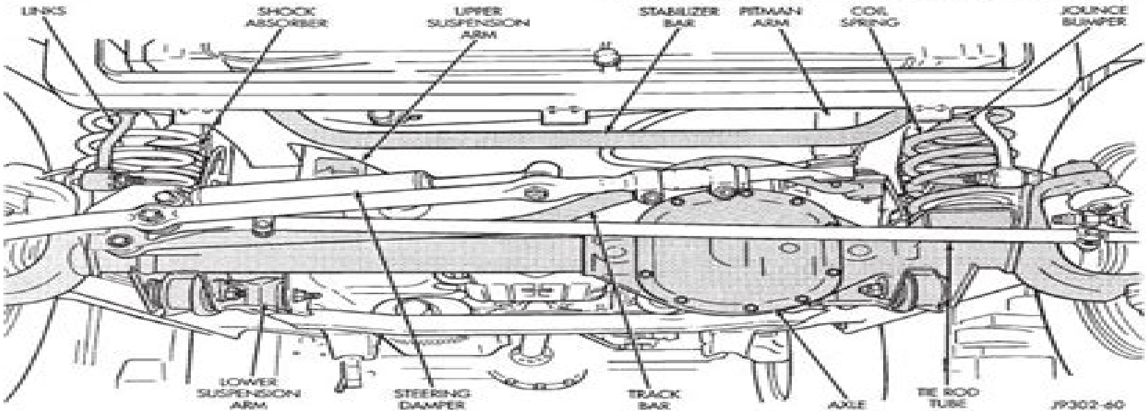
Fig. 1 Front Suspension
