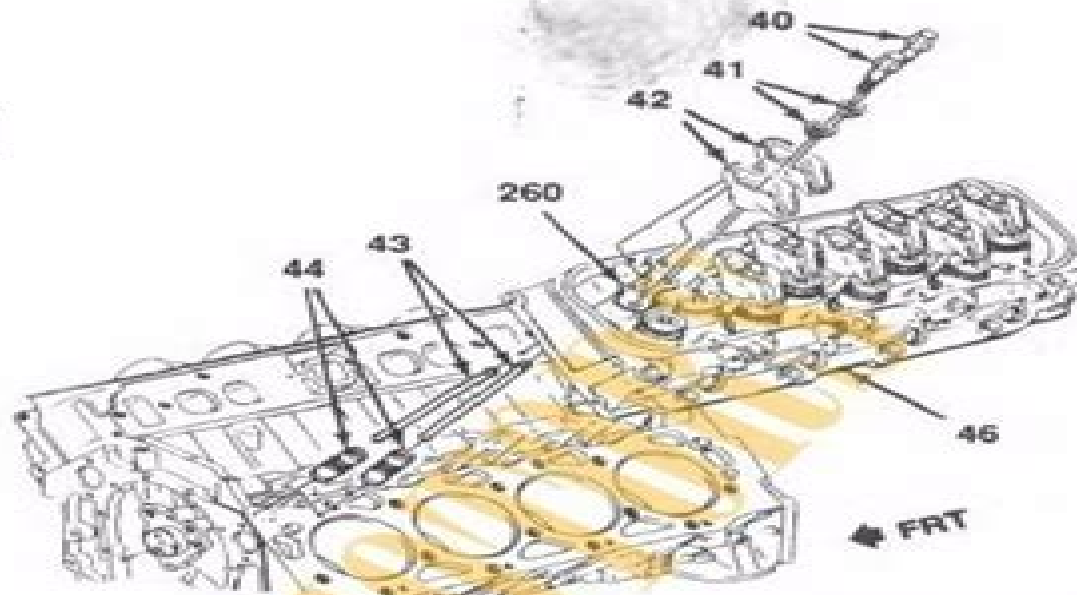
Figure 72—Cylinder Head and Components (7.4L Engines)
