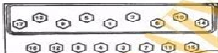
Figure 73—Cylinder Head Bolt Tightening Sequence (5.0L and 5.7L Engines)
