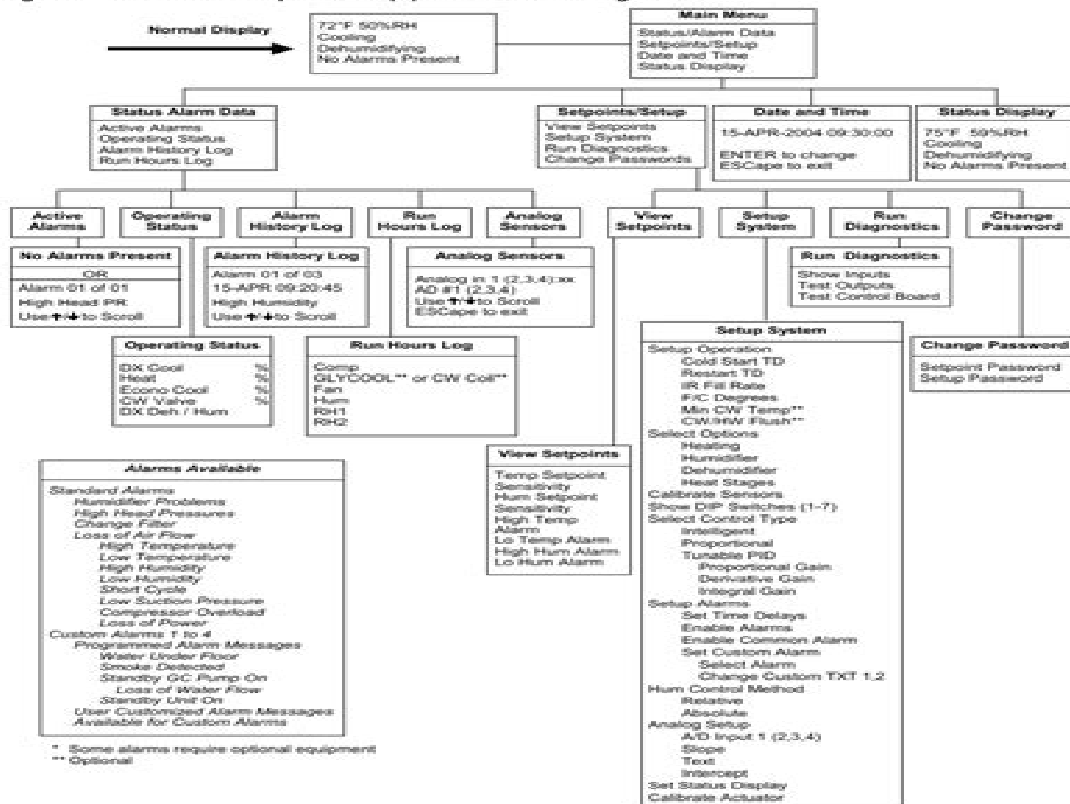
Figure 2 Advanced microprocessor (A) control for Challenger 3000
