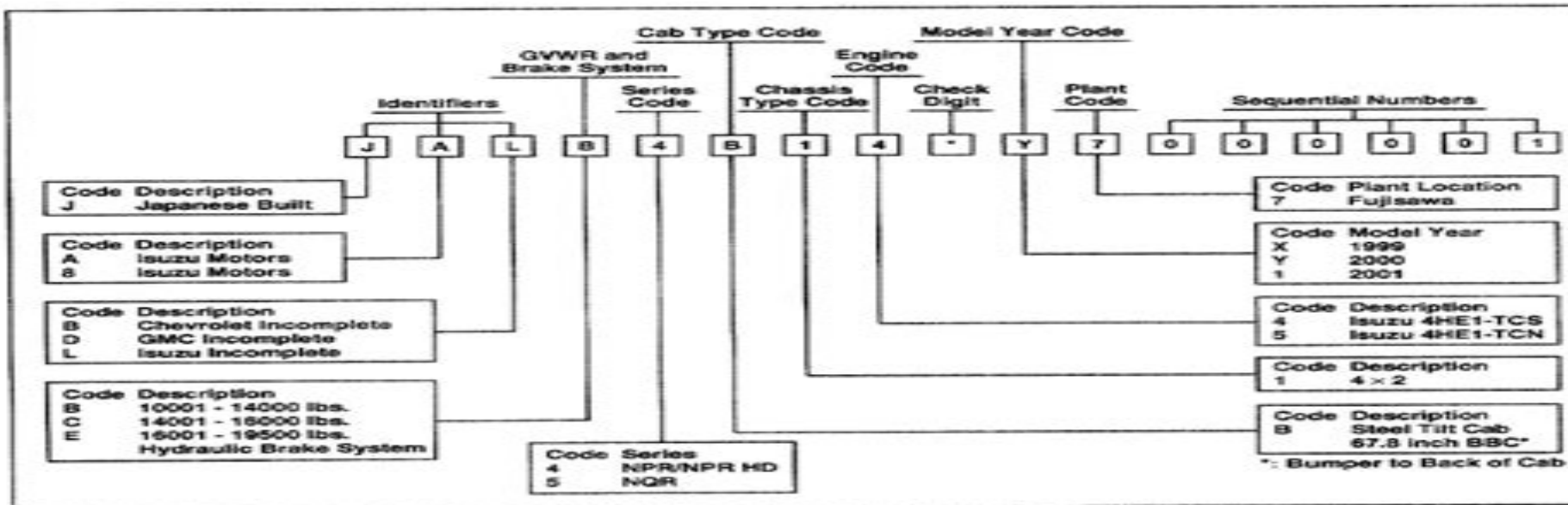
Figure 5. VIN Chart
