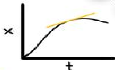
Instantaneous Velocity
