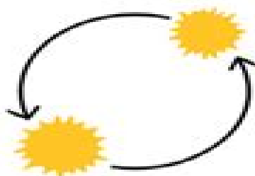
Binary Star
