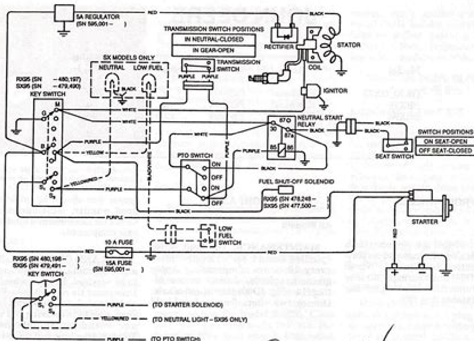
9—Wiring schematic for Models RX95 and SX95.
