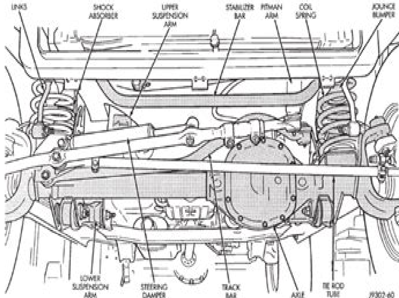
Fig. 1 Front Suspension
