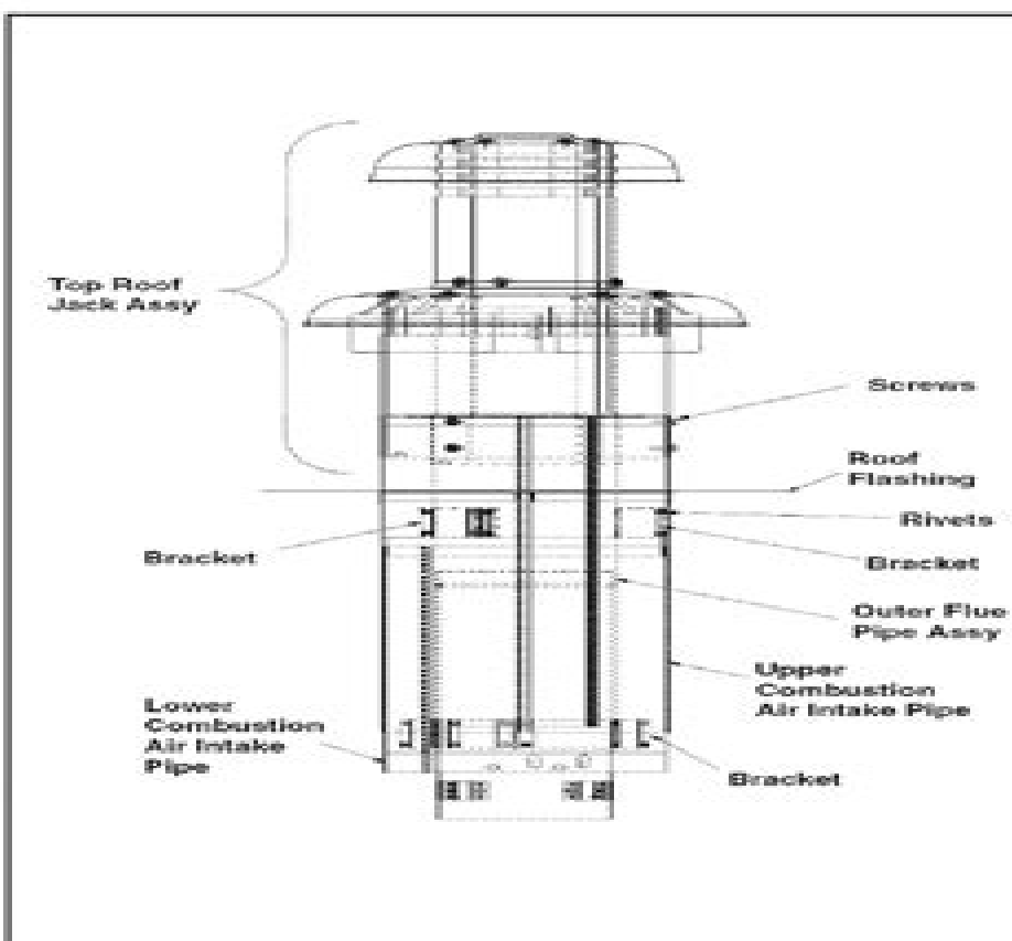
Figure 1. Typical Existing Roof Jack
