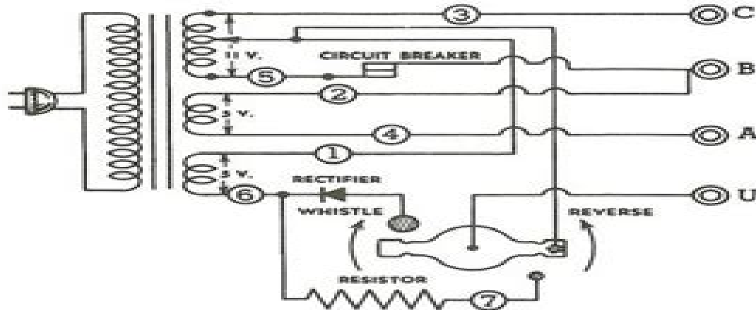
SCHEMATIC WIRING DIAGRAM OF TRANSFORMERS Nos. 1032, 1033, 1032M and 1232
