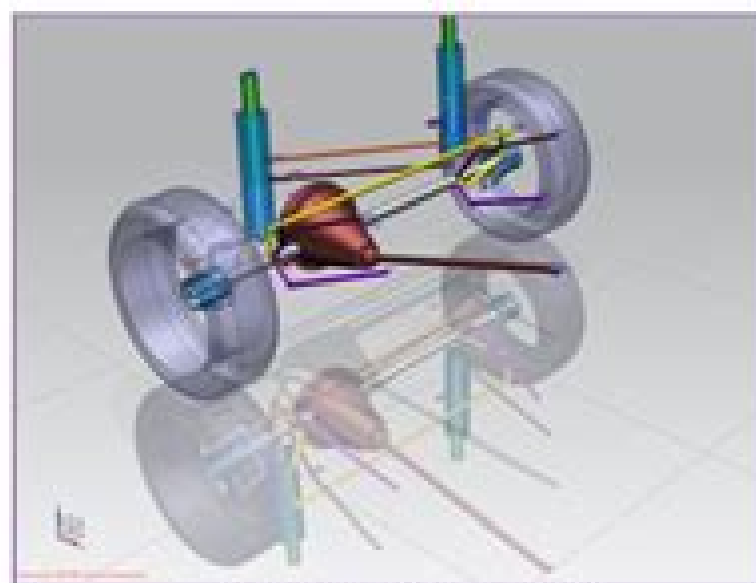
Four Link Solid Front Suspension
