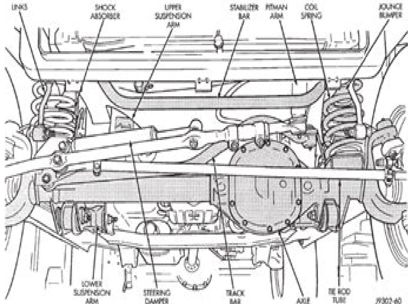
Fig. 1 Front Suspension
