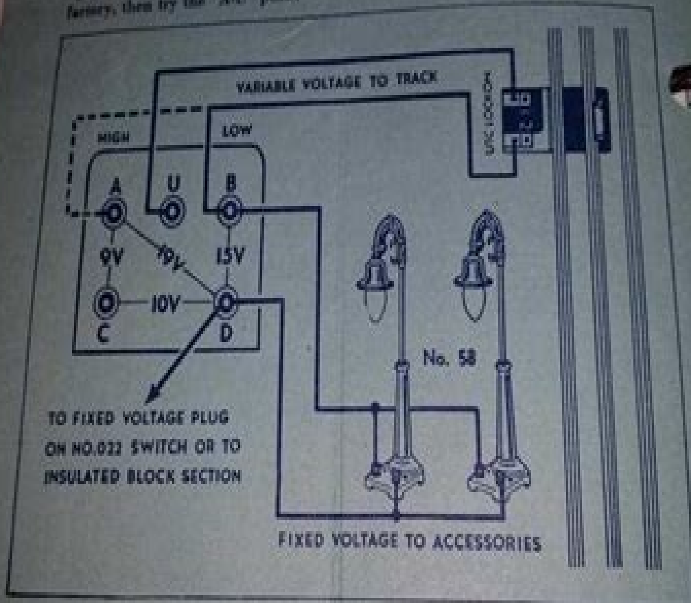
Figure 1 — Connections to "BW" Multi-Control Transformer
