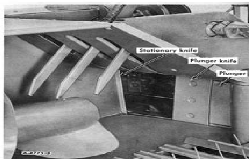
Illustr. 31C - Here the plunger hay knife is shown in position for removal through the feed opening. It is attached to the plunger by means of three bolts (nuts are on the inside of the plunger).
