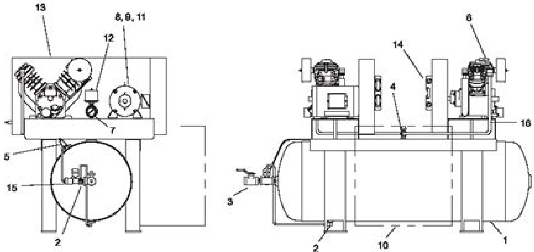
FIGURE 8. TYPICAL DUPLEXER/OMER MOUNTED ELECTRIC PACKAGES.
