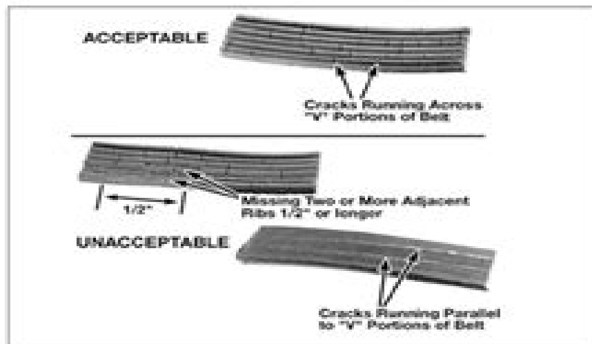
24.4 Small cracks in the underside of a V-ribbed belt are acceptable - lengthwise cracks, or missing pieces that cause the belt to make noise, are cause for replacement
