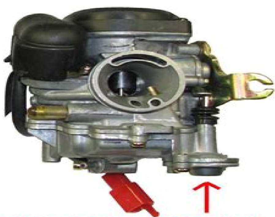
GY6 50cc Carb With Build-in Fuel Pump
