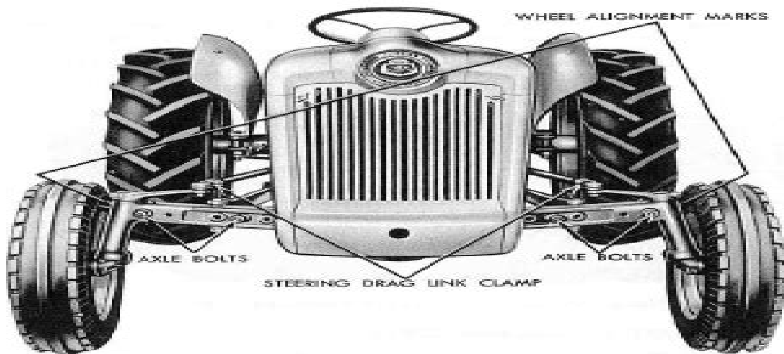
Figure 24 Front Wheel Toe-In Adjustment
