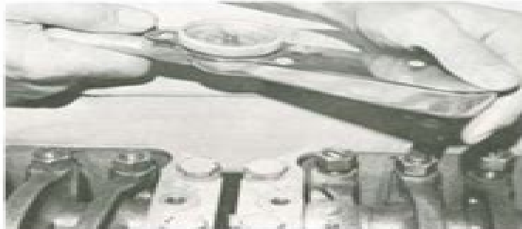
Fig. 14-101, DN114063. Adjusting injector plunger
