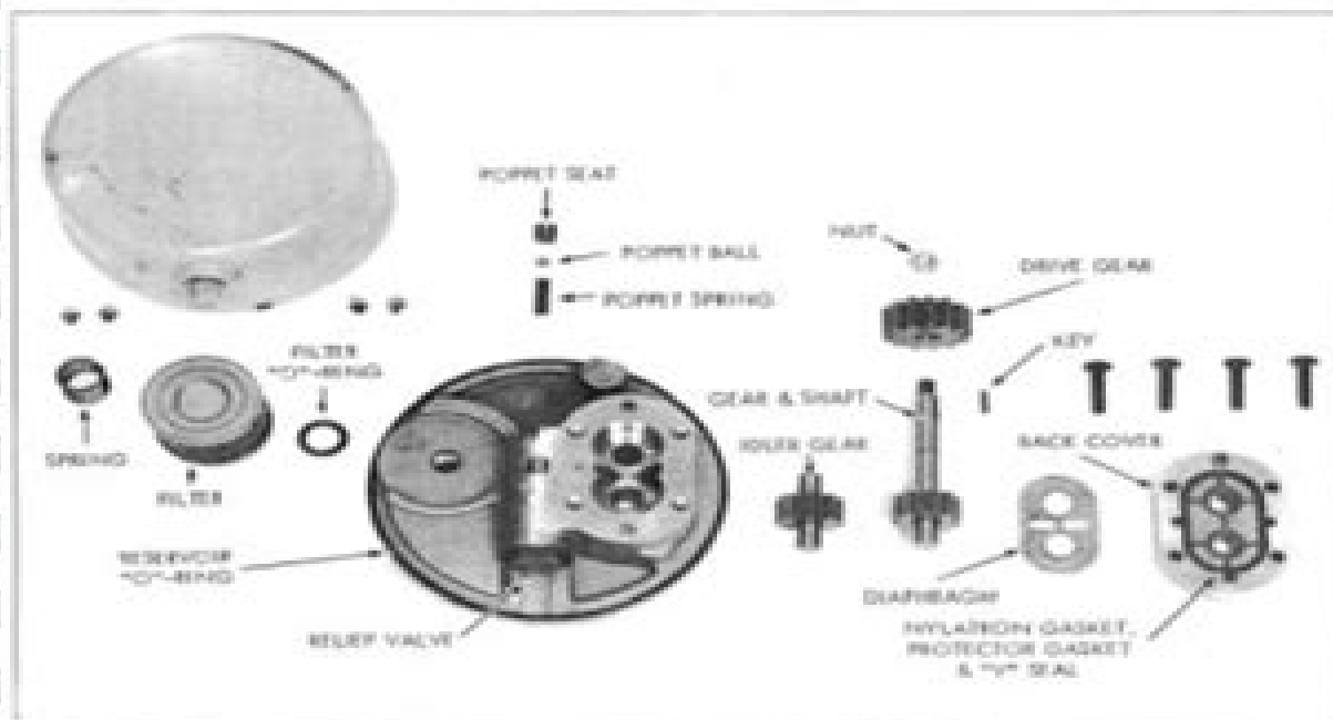
Fig. 4 - Exploded View of Steering Pump - MF 150 - Diesel
