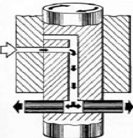
FIG. 113a WORKING PRINCIPLE OF D.P.A. PUMP FIG. 113b
