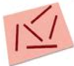
TMD nanoribbons
