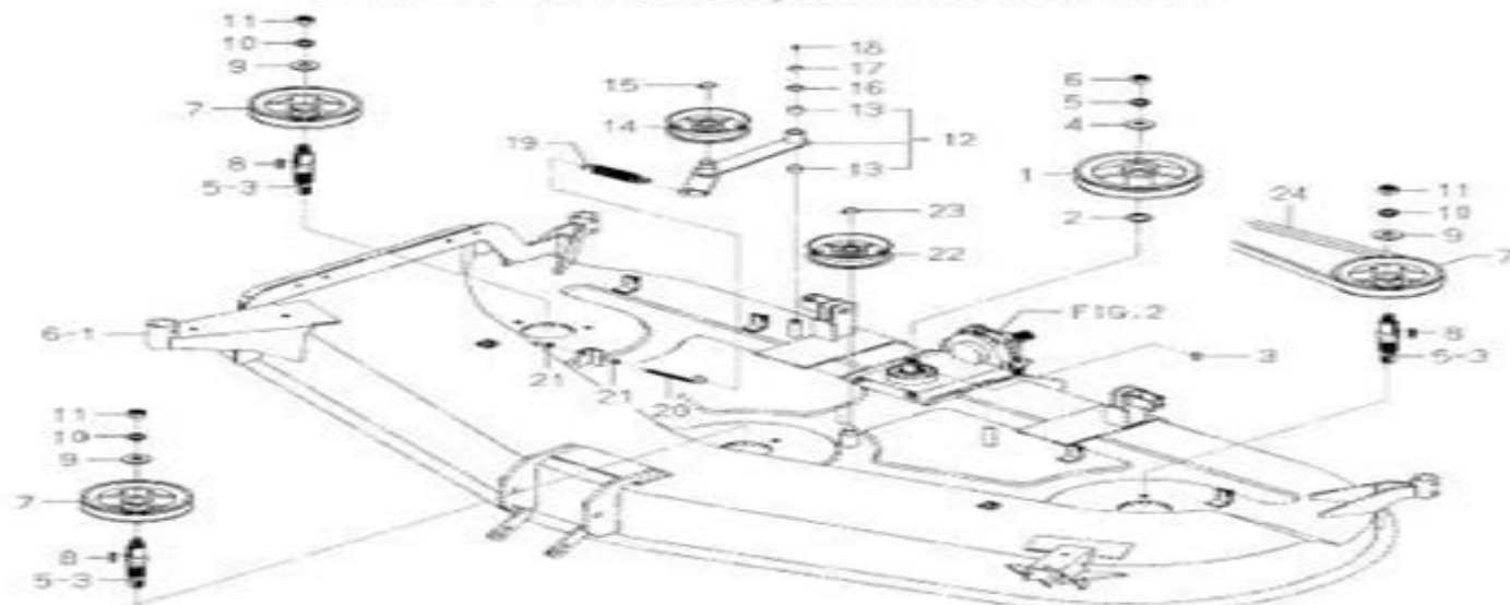
FIG. 3 PULLEY,BELT SYSTEM
