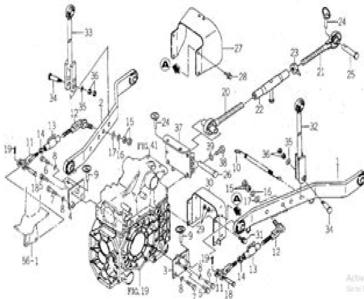
FIG. 47 LINK (3P) SYSTEM
