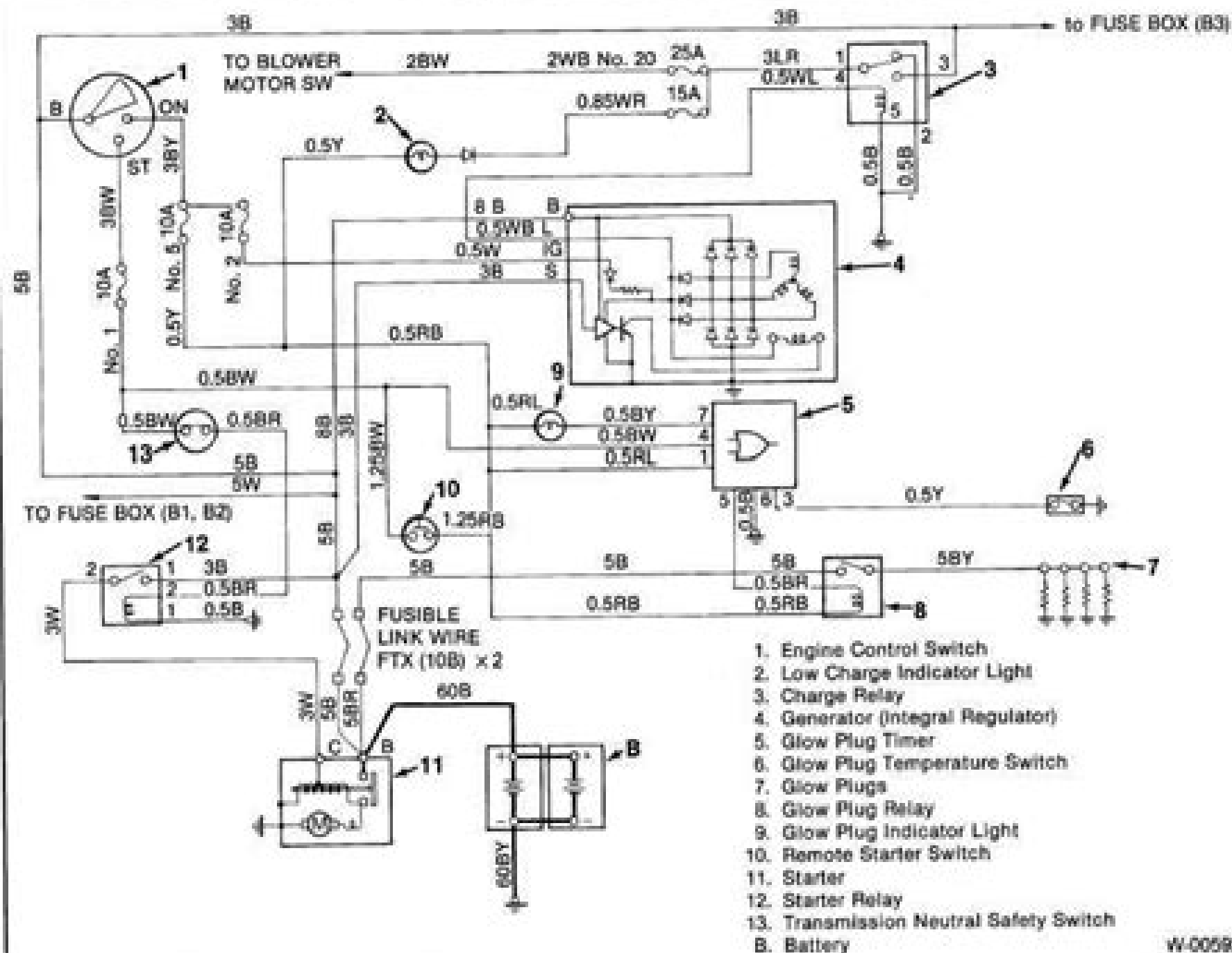
Figure 1. Charging and Starting Systems Circuit Diagram
