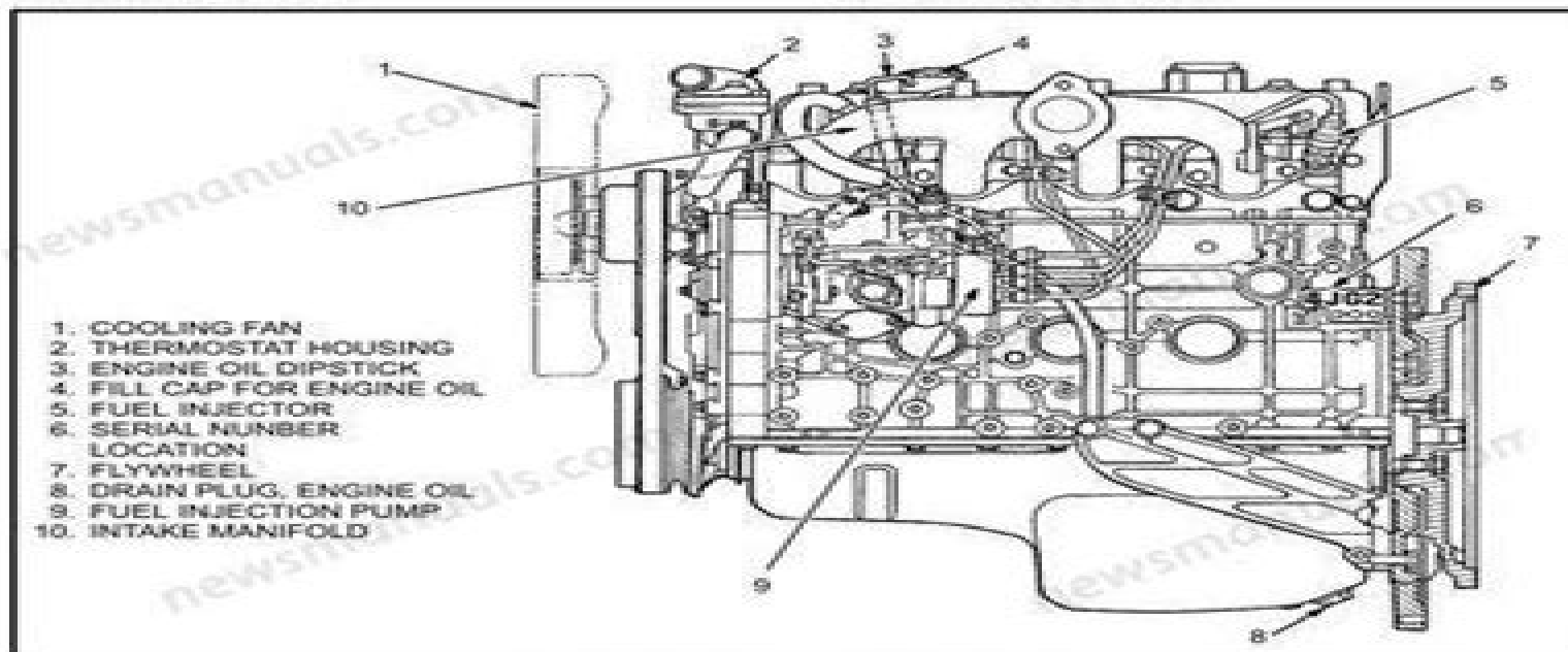
FIGURE 1. ISUZU 4JG2 DIESEL ENGINE
