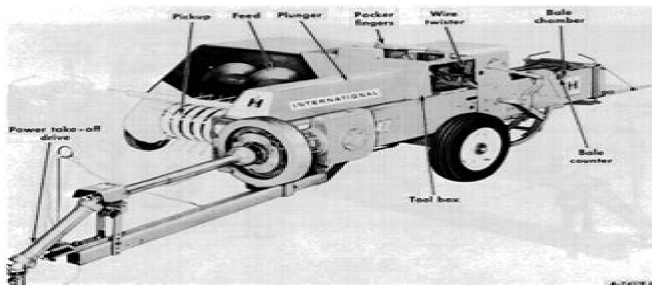
Illustr. 4 Left front view of the 47 Wire Baler.
