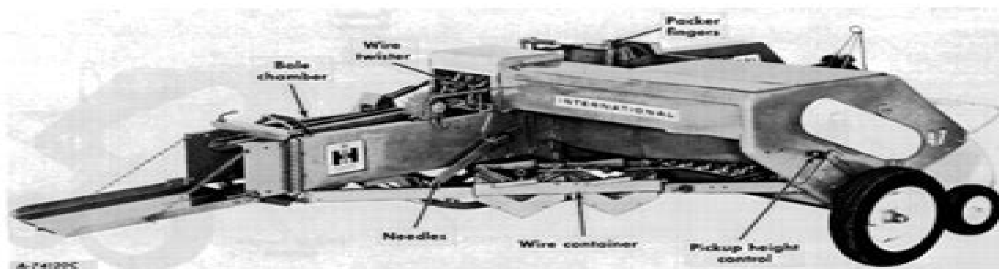
Illustr. 4A Right rear view of the 47 Wire Baler shown with four-cell wire container. Baler can be obtained with two-cell wire container.
