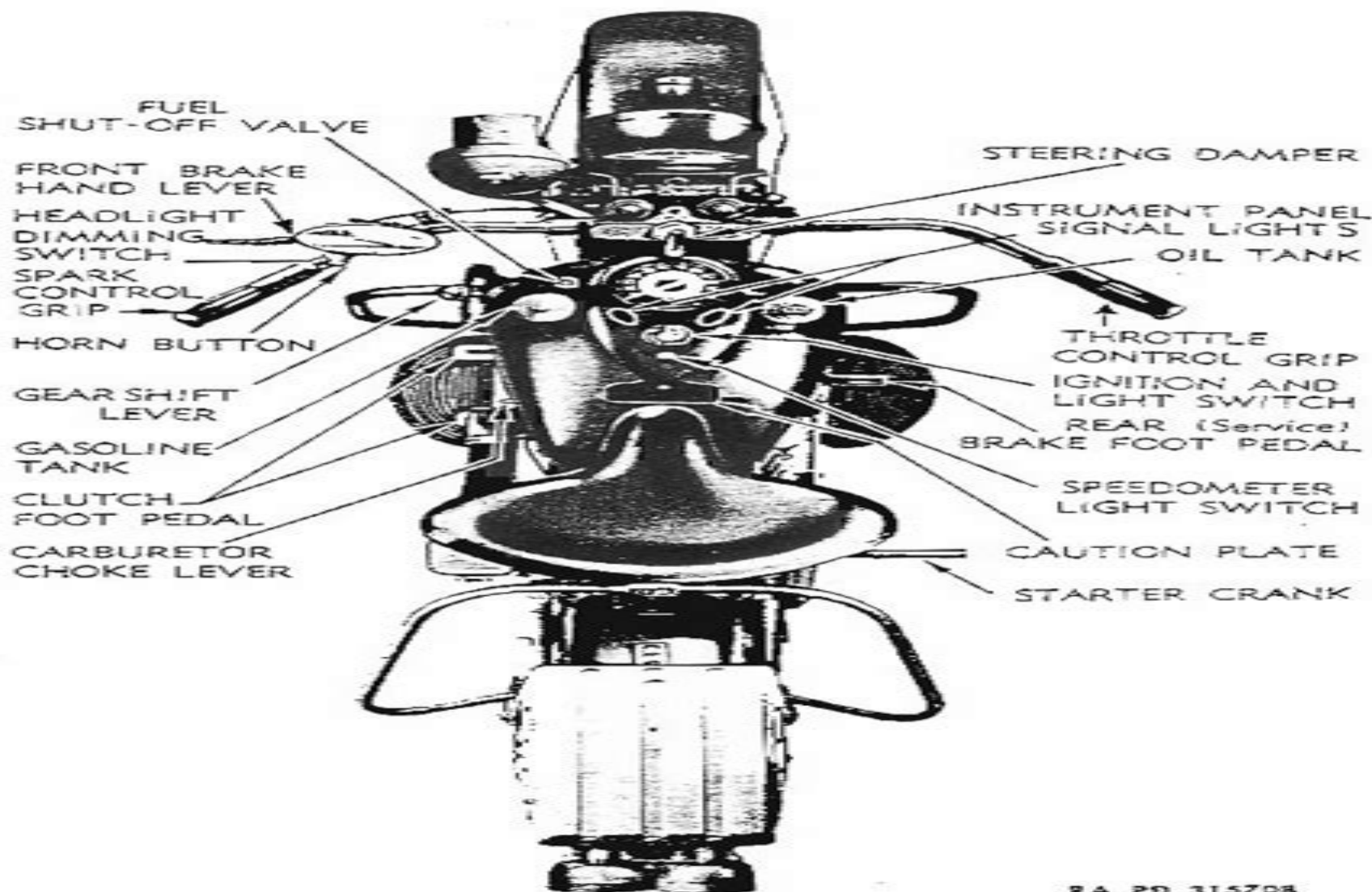
Figure 1—Top View of Motorcycle
