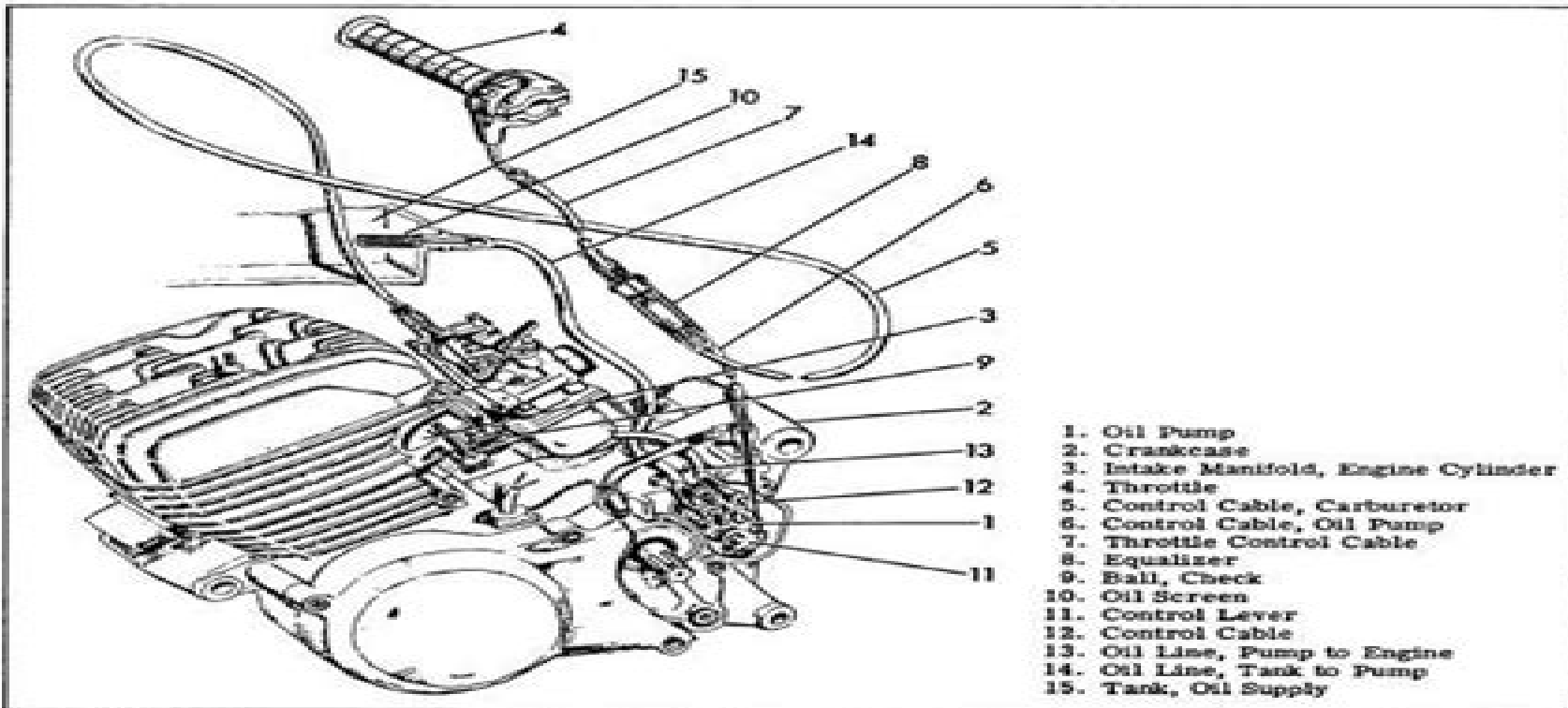
Figure 3.37 Lubrication System
