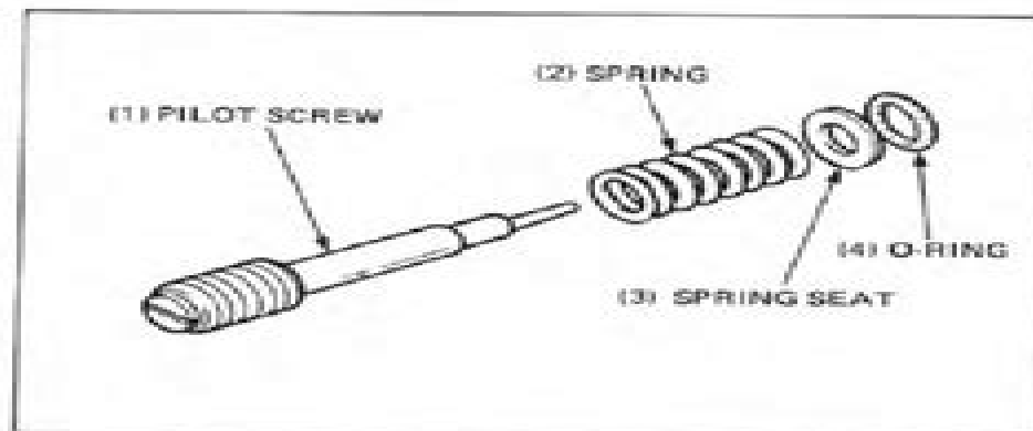
(1) PILOT SCREW
