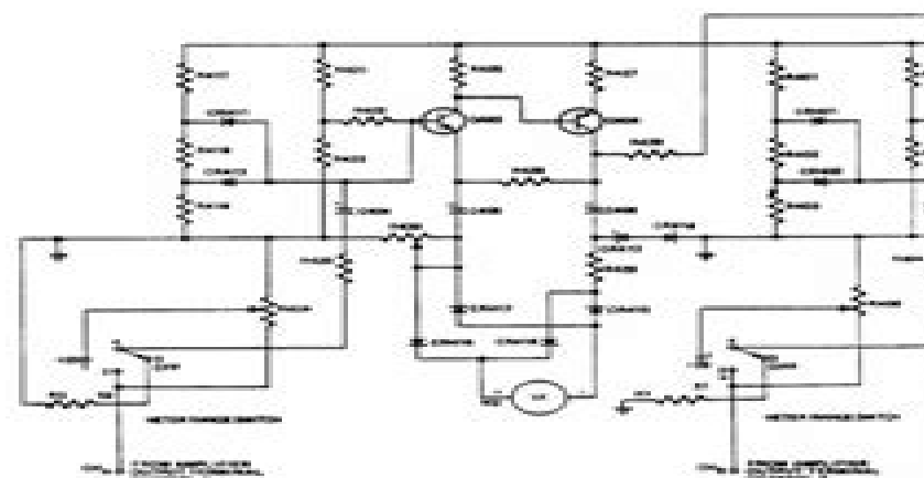
Figure 3. 250 Metering Circuit Simplified Diagram
