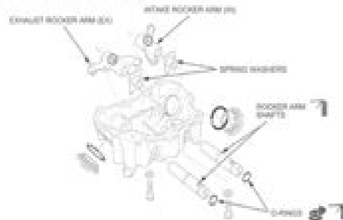
INTAKE ROCKER ARM (IN)
