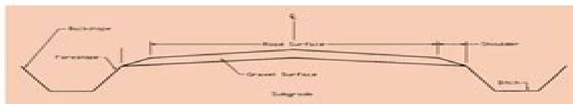
Figure 1: The components of the roadway cross section.
