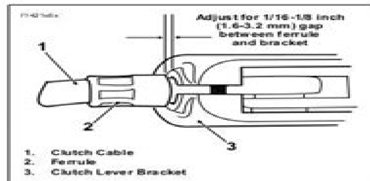
Figure 1-10. Adjust Clutch Free Play
