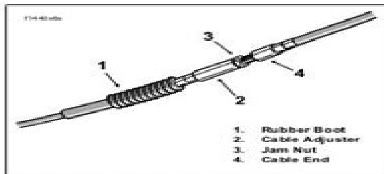
Figure 1-8. Clutch Cable Adjuster Mechanism
