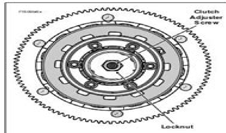
Figure 1-9. Clutch Assembly
