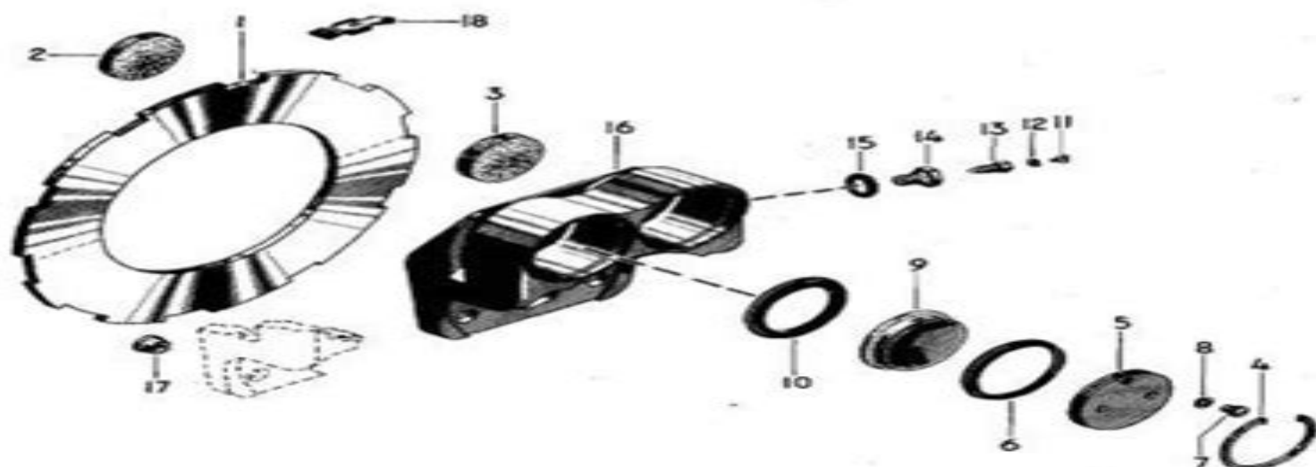
Figure 4. Exploded View, Brake Assembly 511659
