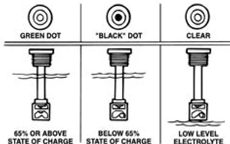
Figure 2 -- Battery Condition
