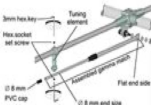
Gamma Match parts list
