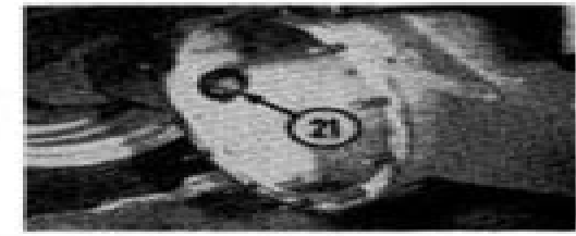
Fig. 11—When removing axle use caution not to damage the oil seal (21) shown. Differential and center hubs been removed for clarity.
