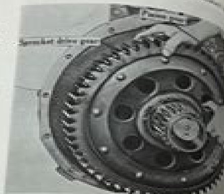
Illustr. 19 - Removing Sprocket Drive Gear (Old Series)
