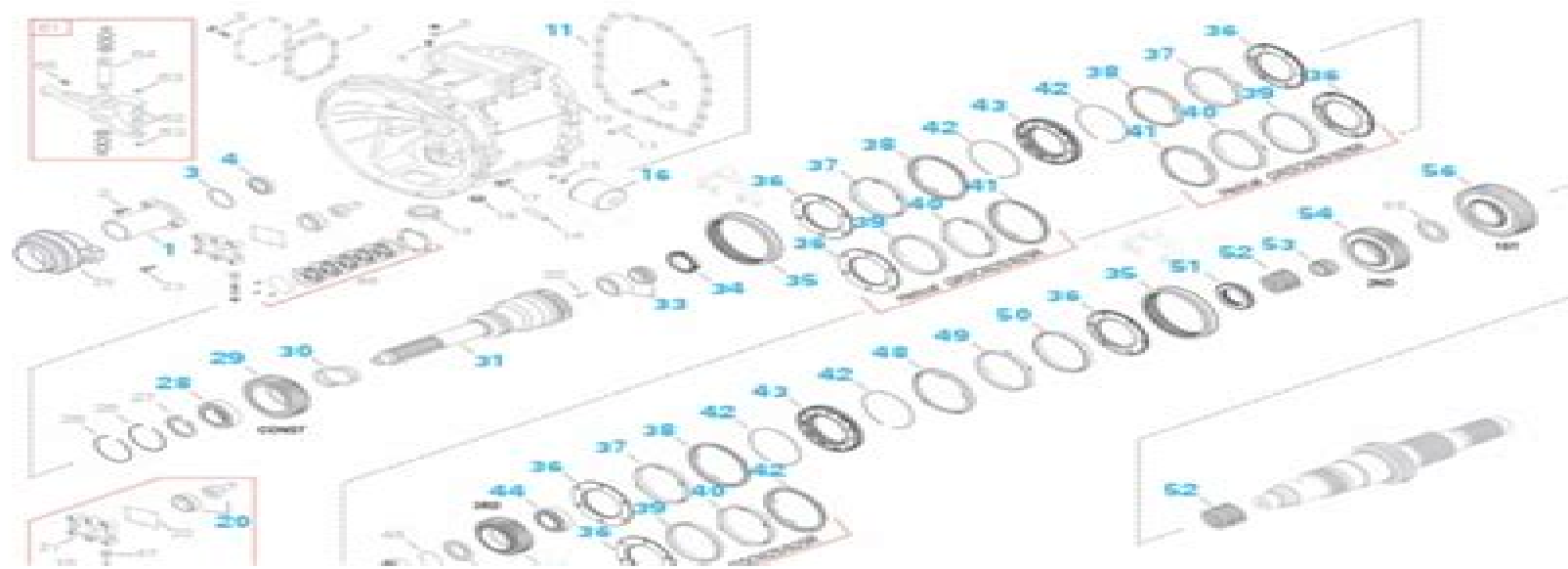
CHART 01 Input Shaft & Main Shaft
