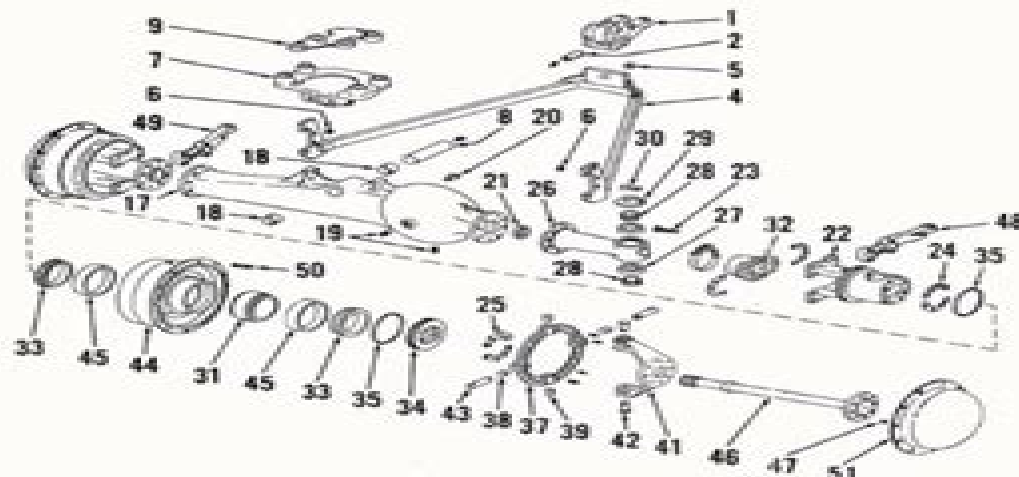
Fig. 7—Exploded view of American Coleman front drive axle used on tractors equipped with "All Wheel Drive". Axle shown is used on tractors with internal steering cylinder.
