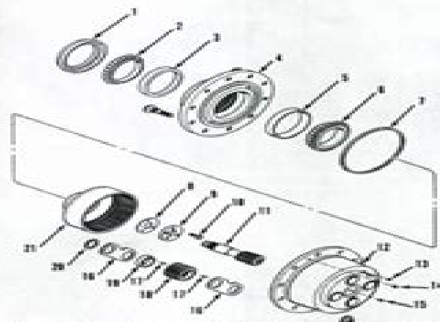
Fig. 6—Exploded view of wheel hub and planetary unit used on front drive axle.
