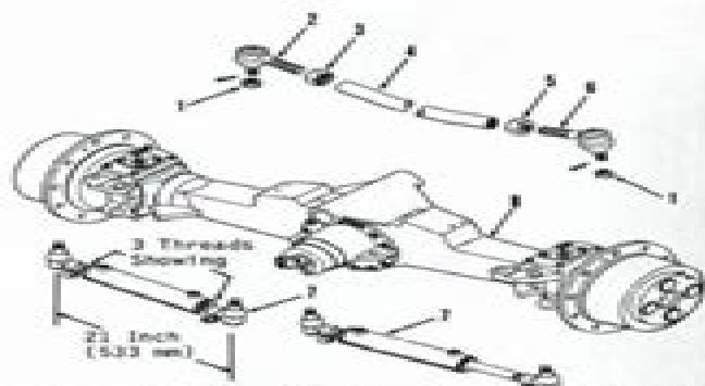
Fig. 5—Front drive axle, tie rod and steering cylinders removed from tractor.
