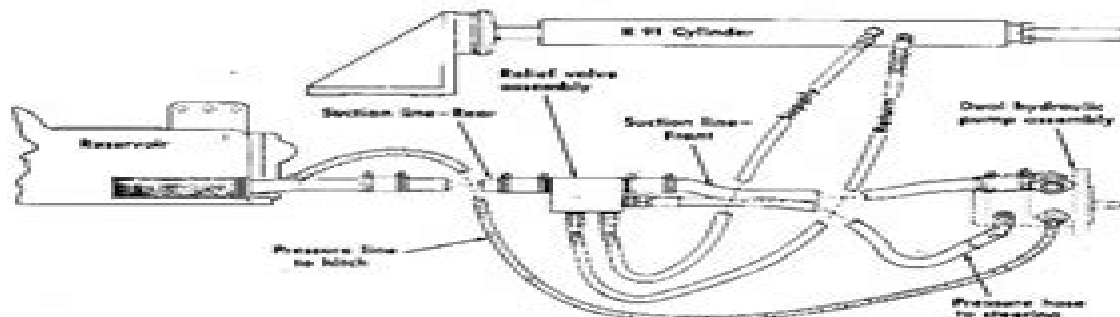
Fig. 12—View showing general arrangement of power steering components used on all Series 354, 364, 384 and Series B-414 S/N 21196 and later. On tractors equipped with R52 cylinder, supply and return hoses are connected to cylinder in reverse of connections shown.
