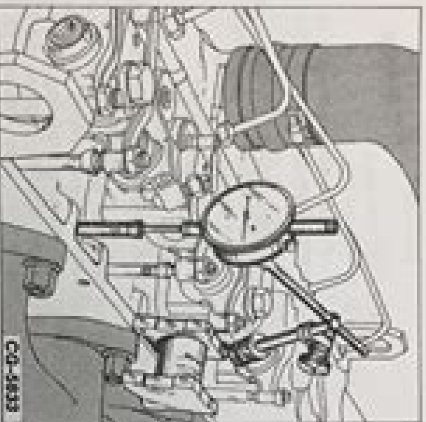
Figure 11 – Checking Cam Lobe Lift (Camshaft in Engine)
