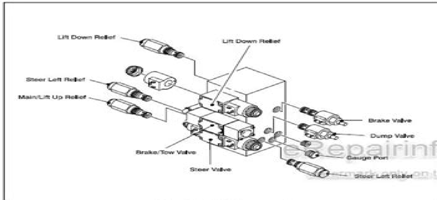
Figure 2-15. Valve Components
